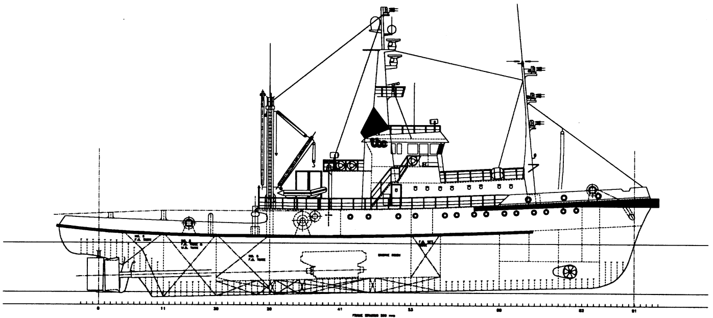
LOWER BRIDGE DECK
