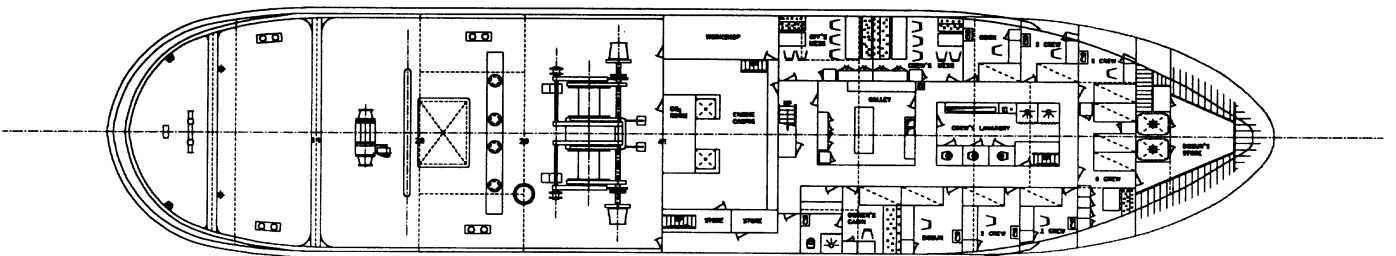
UPPER DECK
